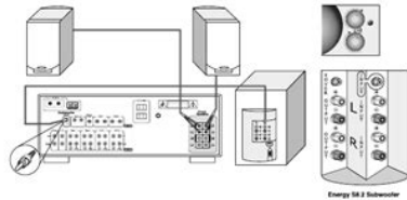
DIAGRAM 3 Using an External Crossover
